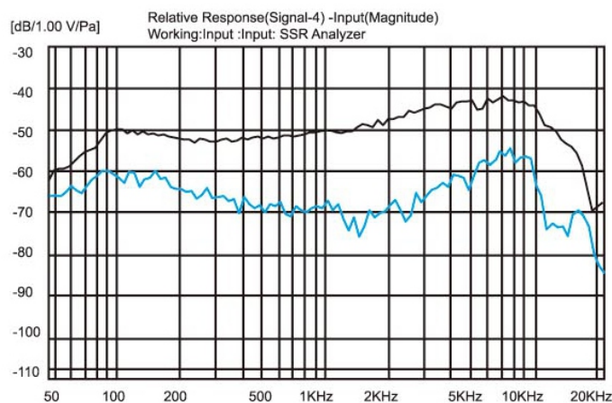
Typical Frequency Response Curve
