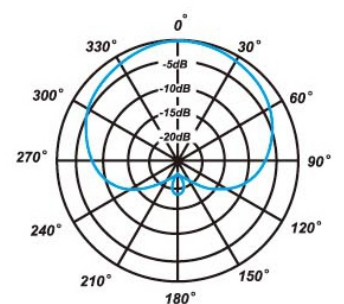
Polar Pattern
