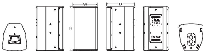
Dimension(W×H×D):245×447×320mm
