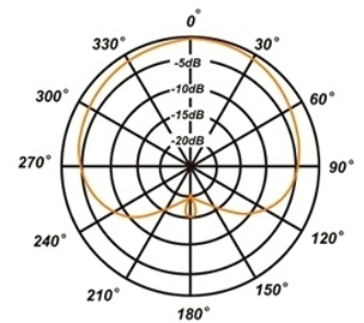
Polar Pattern
