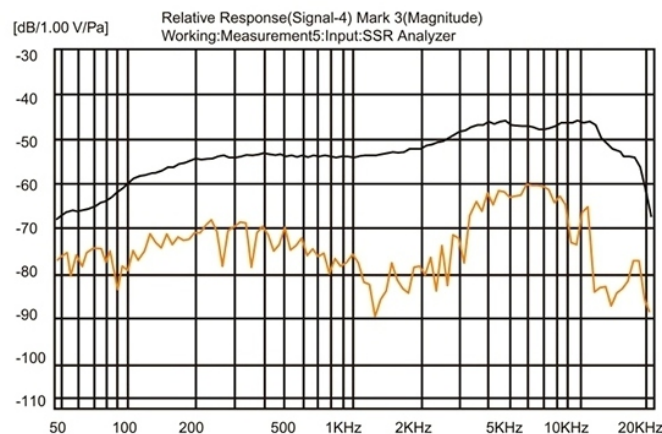
Typical Frequency Response Curve
